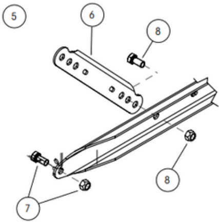
Bolt-on C-channel
